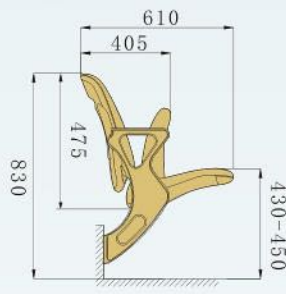
Low-riser Mounted
