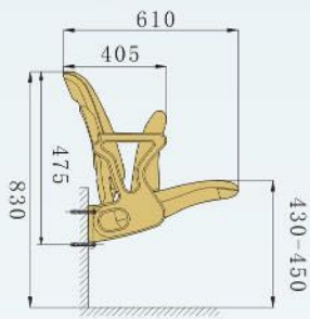
High-riser Mounted
