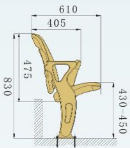
Floor Mounted
